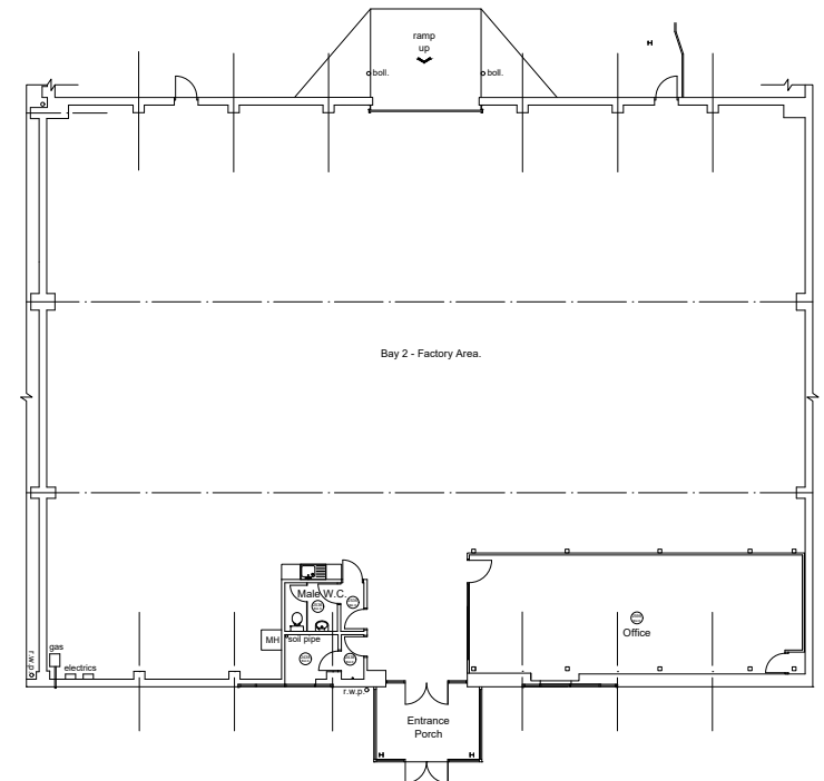
Ground Floor Plan - 7391 sqft. (687 sqm.)
