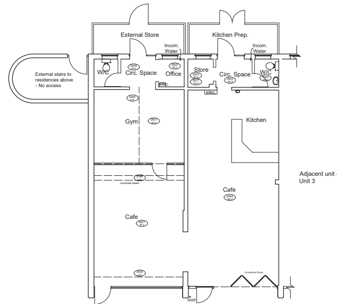
Ground Floor Plan - 140.5m 2 (1512.3ft 2 )
